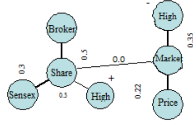
Figure 2: Semantic affinity graph for contextual prior polarity
